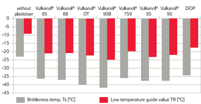
Low-temperature behavior of the Vulkanol® plasticizers in NBR compound
