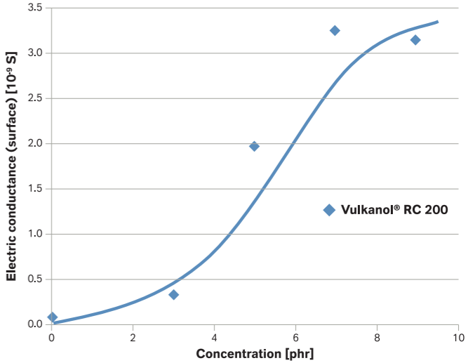
Improvement of electric conductance of a black NBR compound
